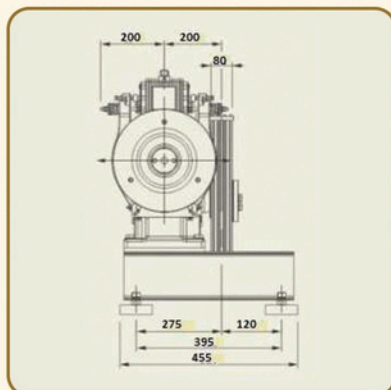
(All Dimensions are mm)
